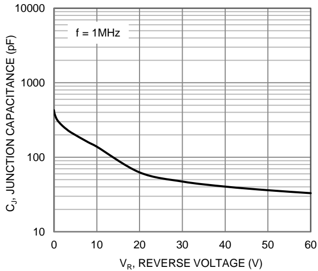
Figure 3. Junction Capacitance vs. Reverse Voltage
