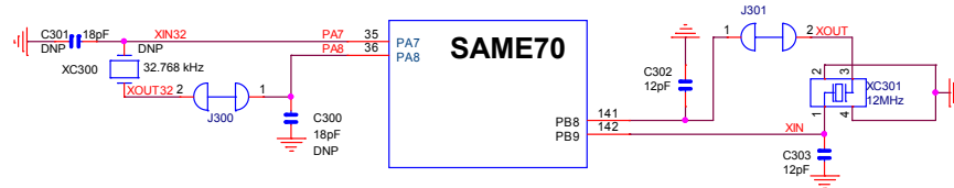
Figure 4-19 SAM E70 Crystals Schematic
