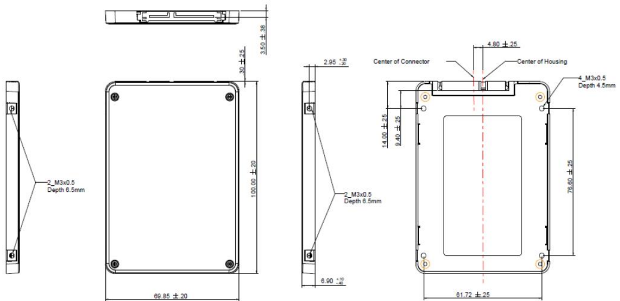
Figure 9-1 Physical Dimensions
