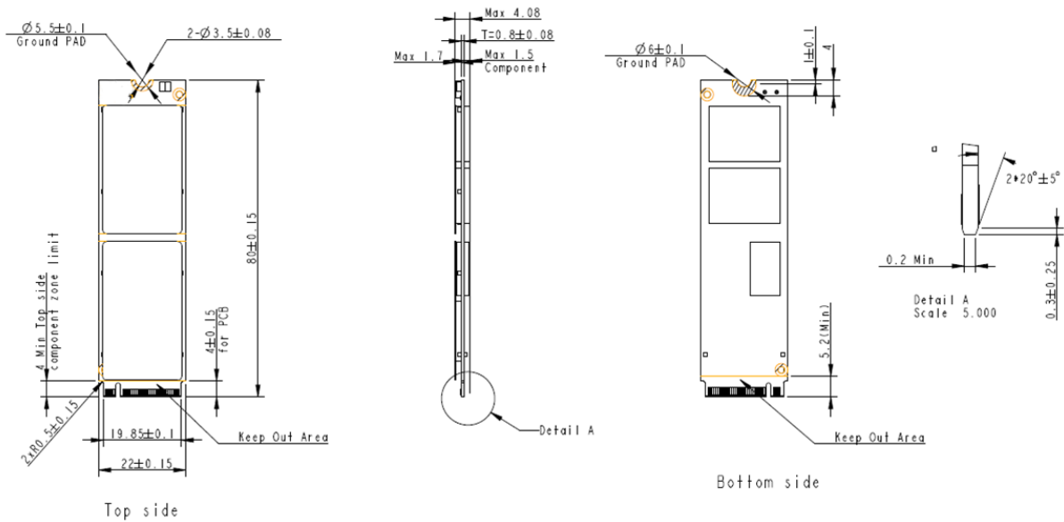
Figure 9-1 Physical Dimensions
