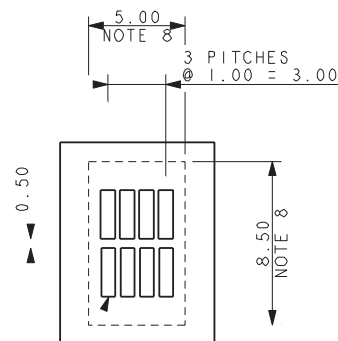
SMT PCB FOOTPRINT
