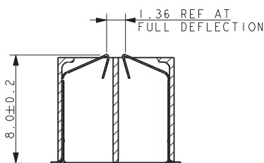
SECTION ON A-A FULL DEFLECTION
