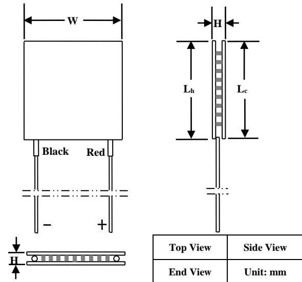
Figure 3. Mechanical Dimensions of Non-sealed TEC
