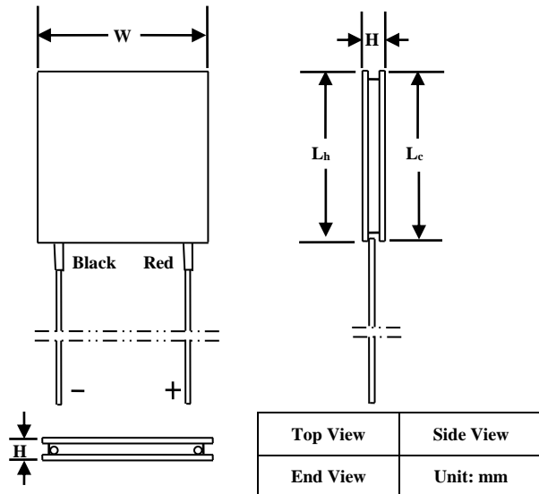
Figure 2. Mechanical Dimensions of Sealed TEC
