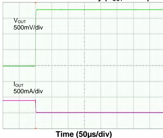
Short Circuit Recovery (V_{OUT} = 1.8V)
