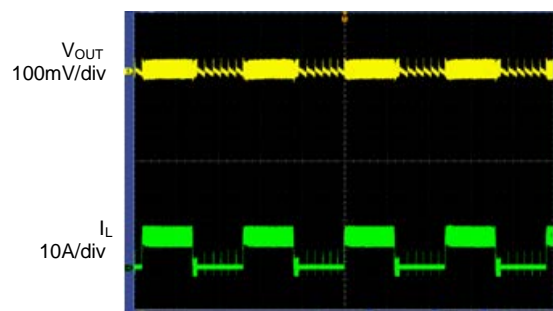
Load Transient Response @ DEM
