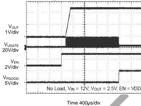
Figure 1. Start-up Behavior of AP3591
