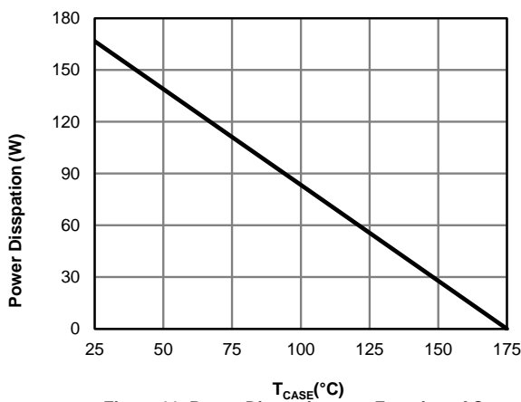
Figure 11: Power Dissipation as a Function of Case
