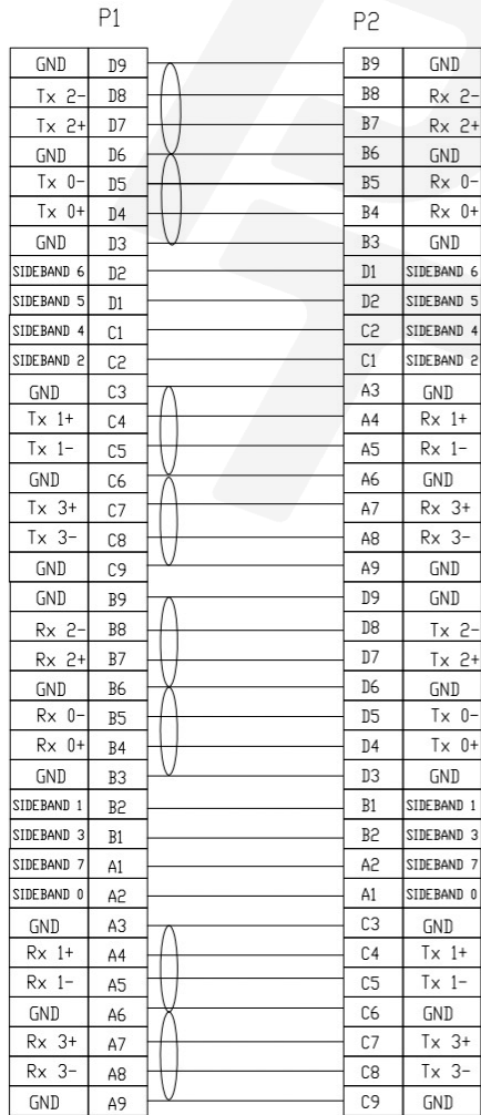
WIRING DIAGRAM
