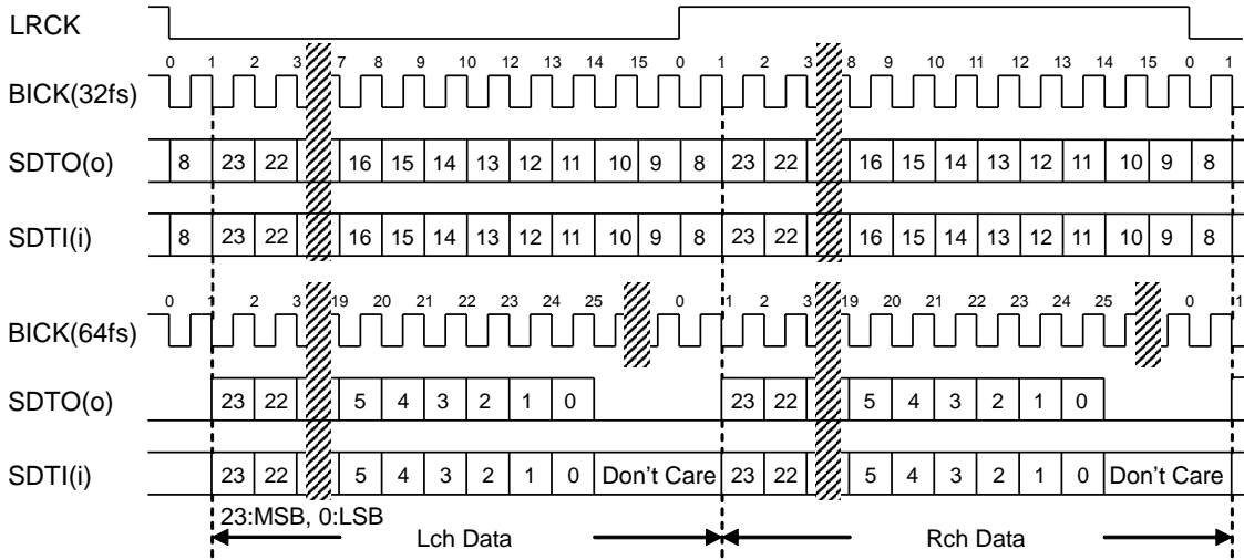
Figure 21. Mode 3 Timing
