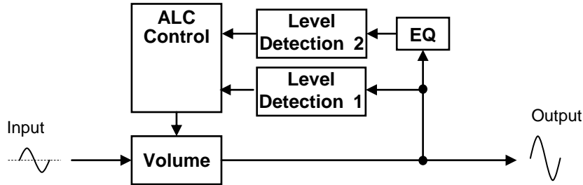
Figure 35. ALC Block
