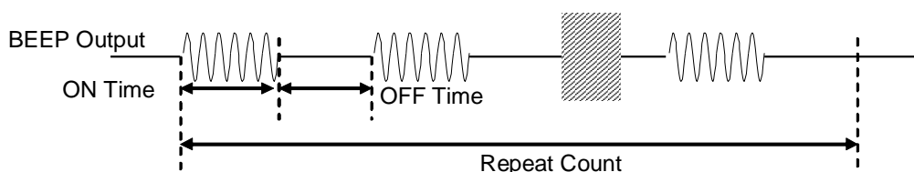
Figure 47. BEEP Output
