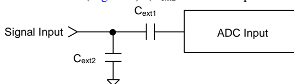
Figure 2. ADC Analog Characteristics Measurement Circuit
