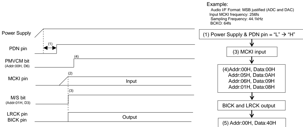
Figure 67. Clock Set Up Sequence (4)
