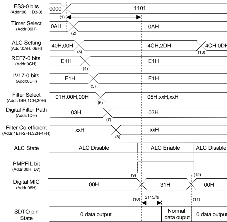
Figure 69. Digital Microphone Input Recording Sequence
