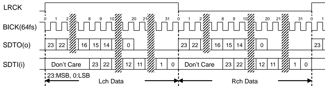
Figure 18. Mode 0 Timing
