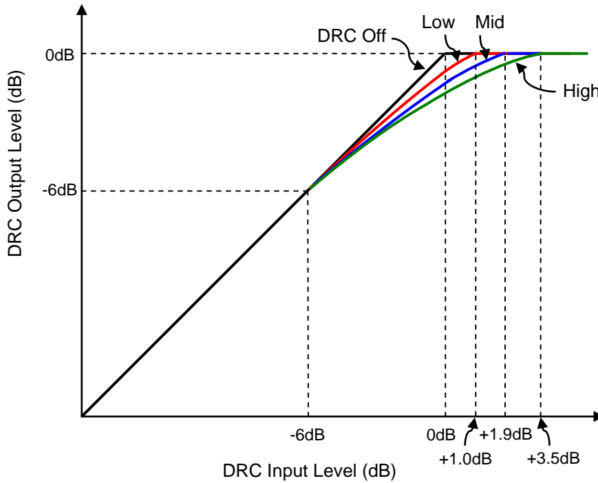
Figure 45. DRC Gain Curve
