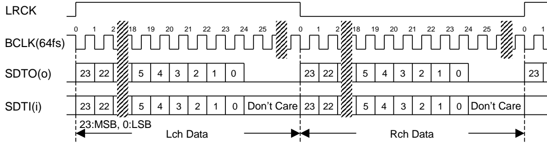
Figure 20. Mode 2 Timing
