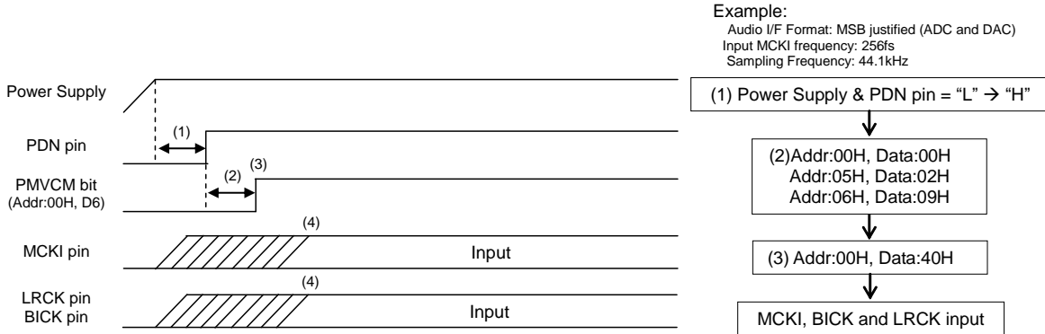
Figure 66. Clock Set Up Sequence (3)
