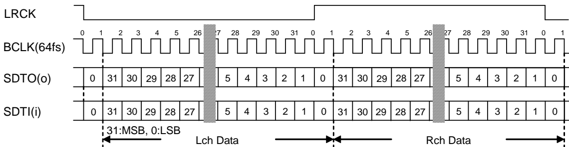
Figure 23. Mode 5 Timing
