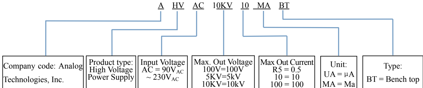
Figure 5. Naming Rules of AHVAC10KV10MABT
