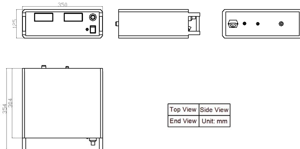
Figure 7. Dimensions for AHVAC10KV10MABT
