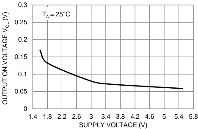
Figure 3. Output On Voltage vs. Supply Voltage
