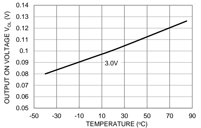
Figure 4. Output On Voltage vs. Temperature
