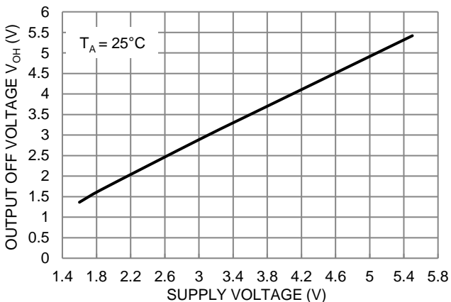
Figure 5. Output Off Voltage vs. Supply Voltage
