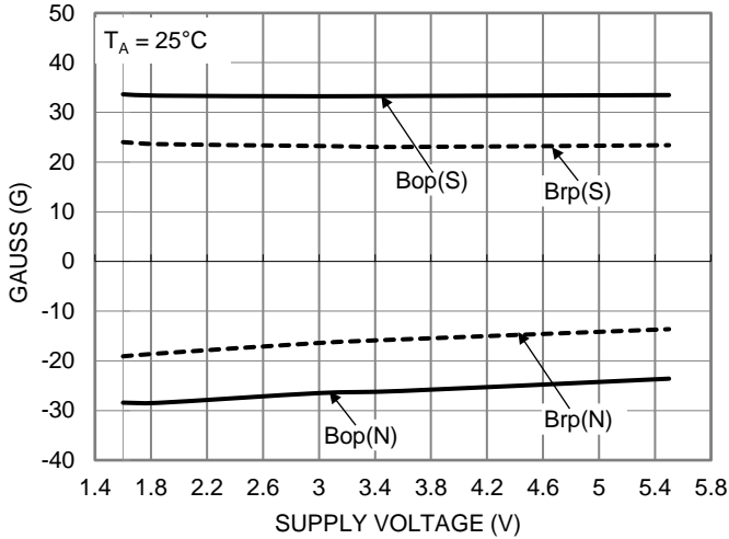
Figure 7. Switch Points vs Supply Voltage
