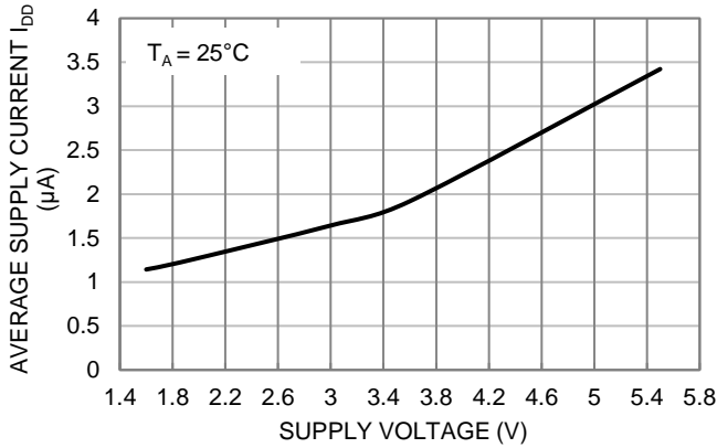
Figure 1. I_{DD(AVG)} vs. Supply Voltage
