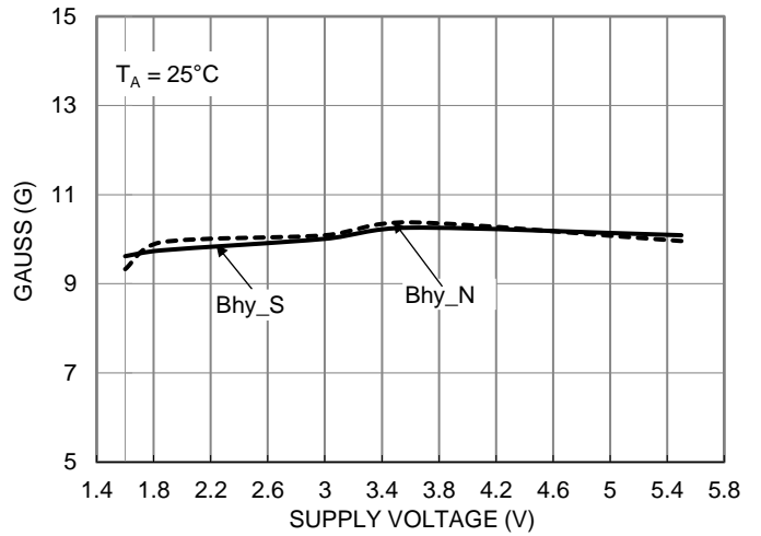
Figure 8. Hysteresis B_{HY} vs Supply Voltage
