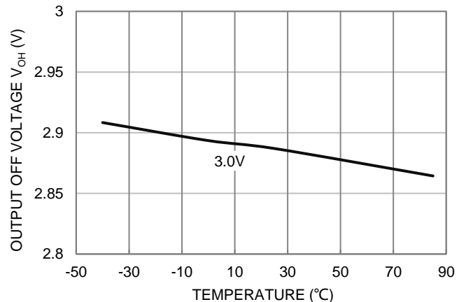
Figure 6. Output Off Voltage vs. Temperature
