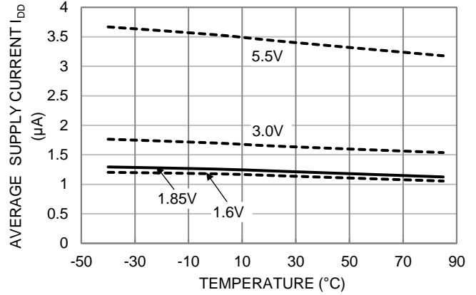
Figure 2. I_{DD(AVG)} vs. Temperature
