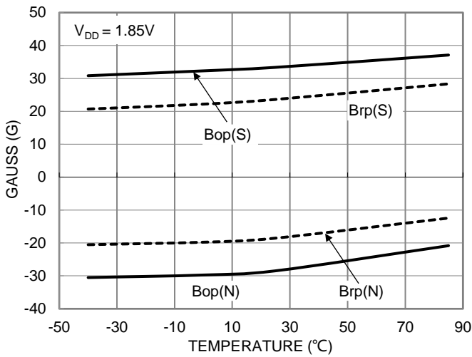
Figure 9. Switch Points vs Temperature
