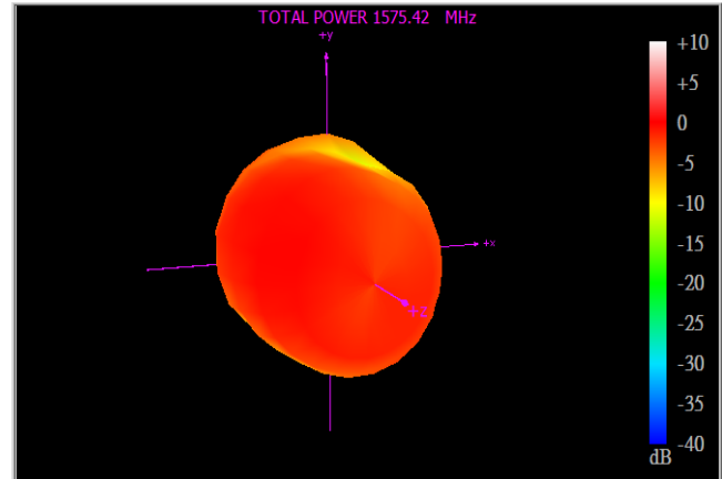
1575.42MHz
