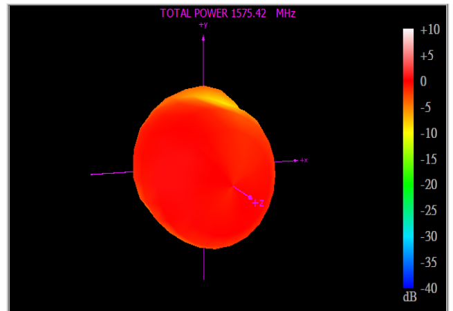
1575.42MHz
