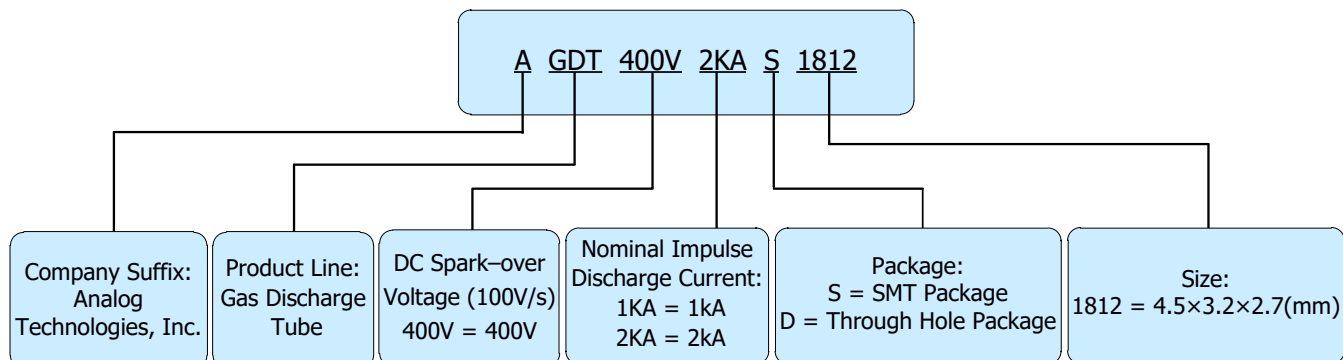
Naming Principle of AGDT400V2KAS1812
