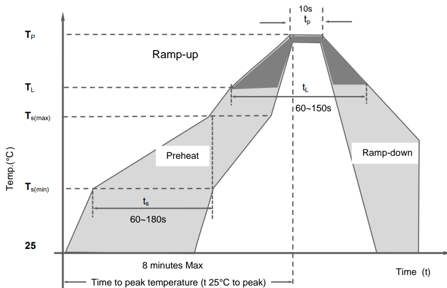
Figure 9. Reflow Soldering
