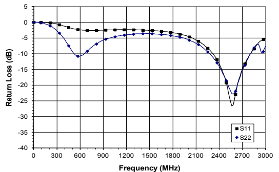
Figure 35: Return Loss vs. Frequency
