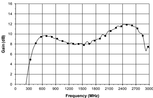
Figure 34: Gain vs. Frequency
