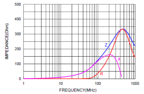
AFBC-Q0805G-121
