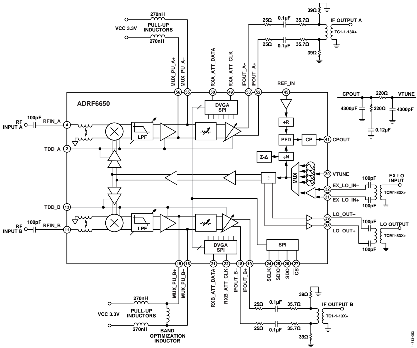
Figure 53. Basic Connections Diagram
