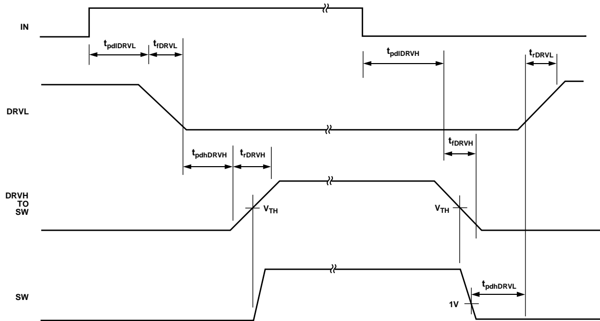
Figure 3. Timing Diagram
