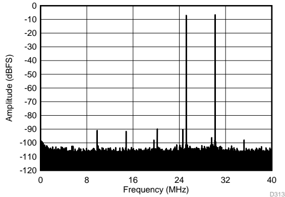
f_{IN1} = 185\text{ MHz} , f_{IN2} = 190\text{ MHz} , \text{IMD3} = 90\text{ dBFS} , each tone at -7\text{ dBFS}
