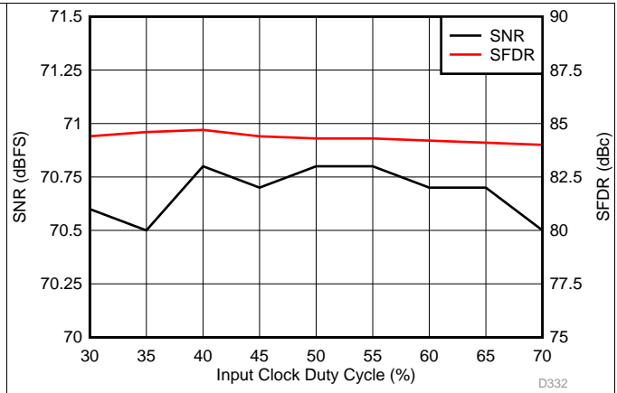
Figure 65. Performance vs Clock Duty Cycle (150 MHz)
