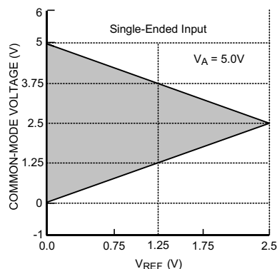
Figure 12. V_{CM} range for single-ended operation
