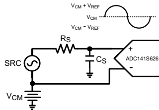
Figure 10. Single-Ended Input
