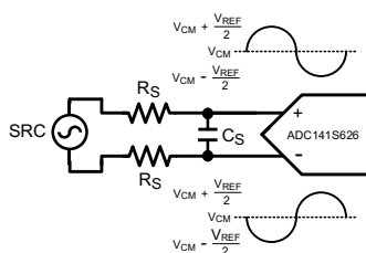
Figure 9. Differential Input
