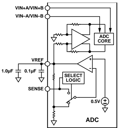
Figure 46. Internal Reference Configuration
