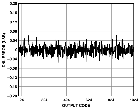
Figure 14. AD9204-80 DNL with f_{IN} = 9.7 MHz
