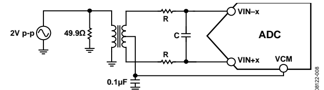
Figure 42. Differential Transformer-Coupled Configuration
