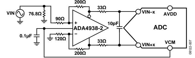
Figure 41. Differential Input Configuration Using the ADA4938-2
