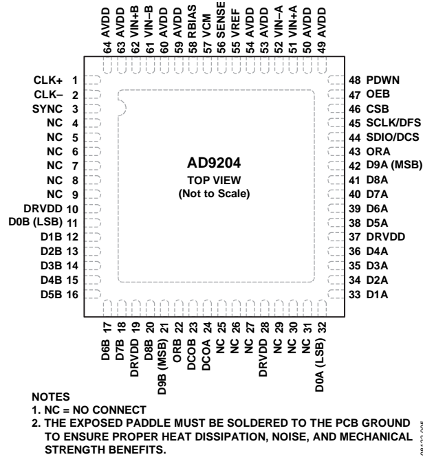
Figure 5. Pin Configuration
