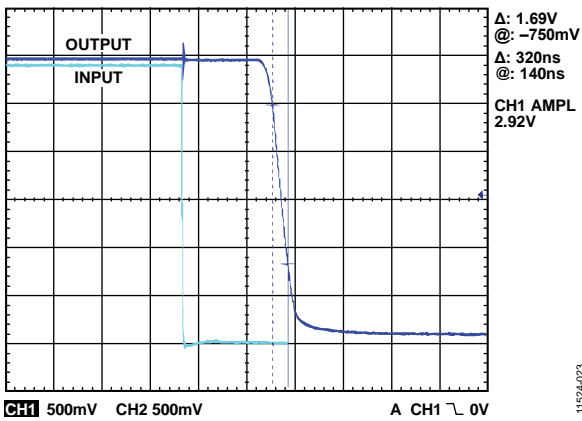
Figure 17. Large Signal Negative Edge Response, V_{SY} = \pm 15.0\text{ V} , T_A = 175^\circ\text{C}
