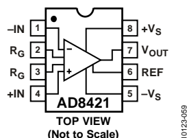
Figure 64. Pin Configuration Diagram
