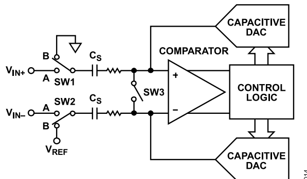
Figure 17. ADC Conversion Phase
