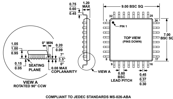
Figure 48. 32-Lead Thin Quad Flat Package [TQFP] (SU-32-2) Dimensions shown in millimeters
