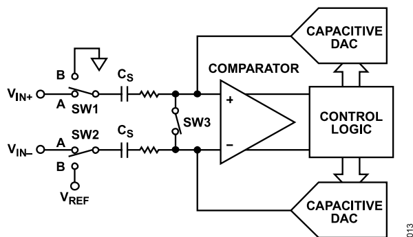
Figure 16. ADC Acquisition Phase
