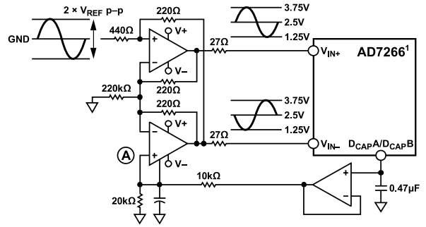
Figure 27. Dual Op Amp Circuit to Convert a Single-Ended Bipolar Signal into a Differential Unipolar Signal
