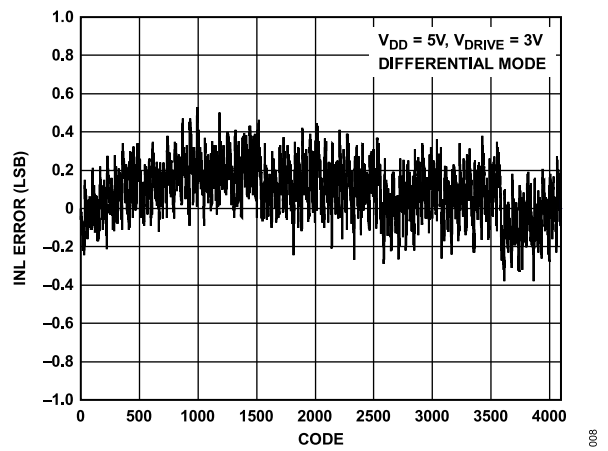
Figure 9. Typical INL
