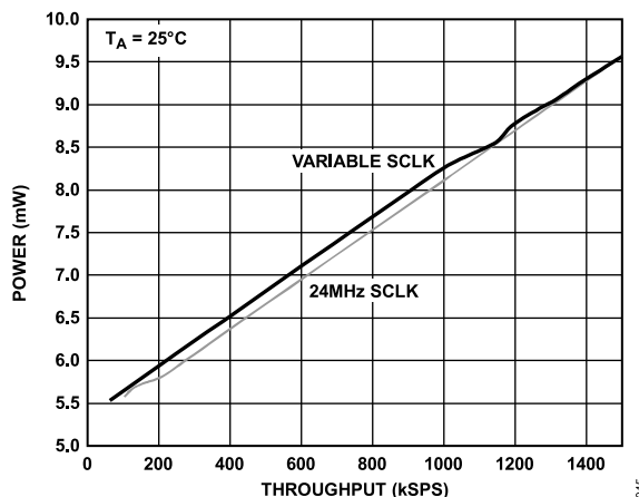
Figure 39. Power vs. Throughput in Normal Mode with V_{DD} = 3 V
