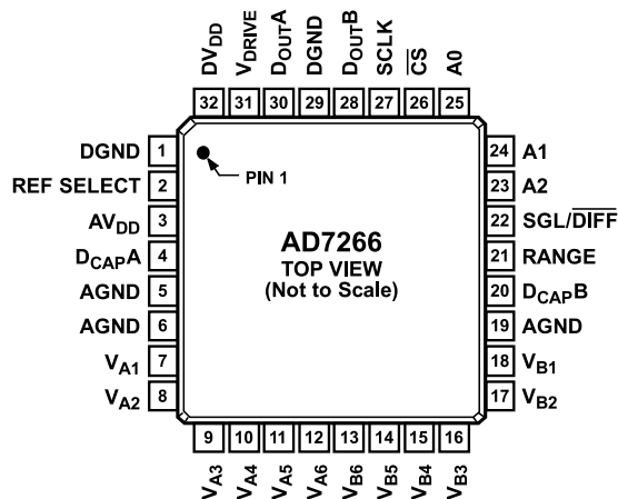
Figure 3. 32-Lead TQFP
