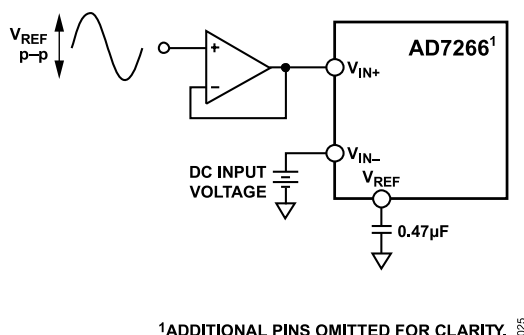
Figure 30. Pseudo Differential Mode Connection Diagram
