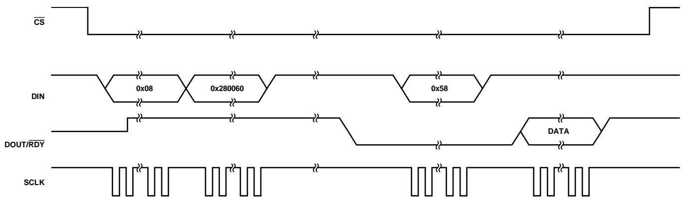
Figure 21. Single Conversion
