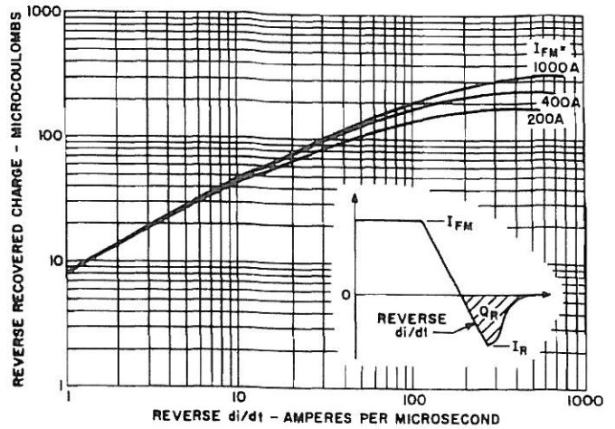
8. TYPICAL RECOVERED CHARGE (T J = 175°C) FOR PARTS SUPPLIED VIA A398-X9 PART NUMBER. GRAPH 8 REPRESENTS A MAXIMUM RECOVERED CHARGE (T J = +175°C)
