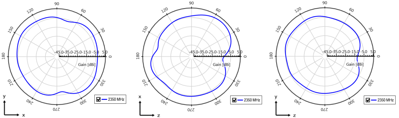
High Band measured at 2350 MHz
