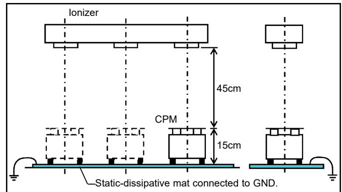
Figure 9. Position of Overhead Air Ionizer and CPM
