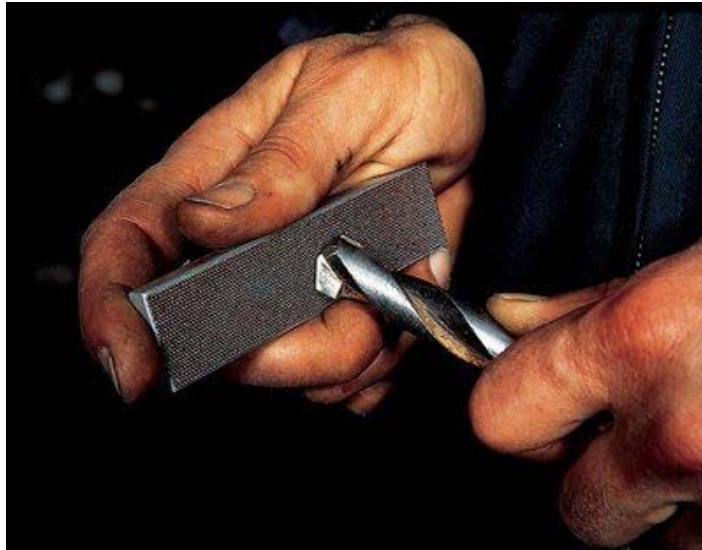
Micron graded flexible diamond abrasive, bonded to a rigid block— excellent for stone faceting and tool sharpening
