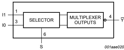
Fig. 3. Functional diagram
