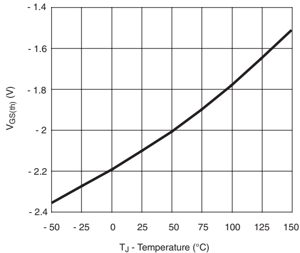
Threshold Variance
