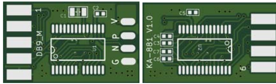
PCBA: KA-881 REV1.0(IC: FT232RL+ZT213LEEA)
