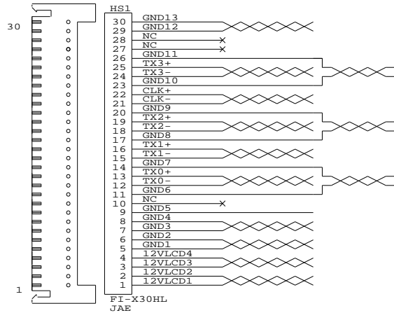
PANEL SIDE
