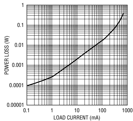
Figure 3. Power Lost vs Load Current
