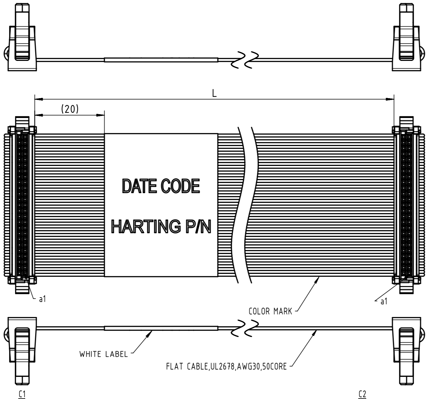
HAR-FLEX 50P FEMALE CONNECTOR WITH STRAIN RELIEF
