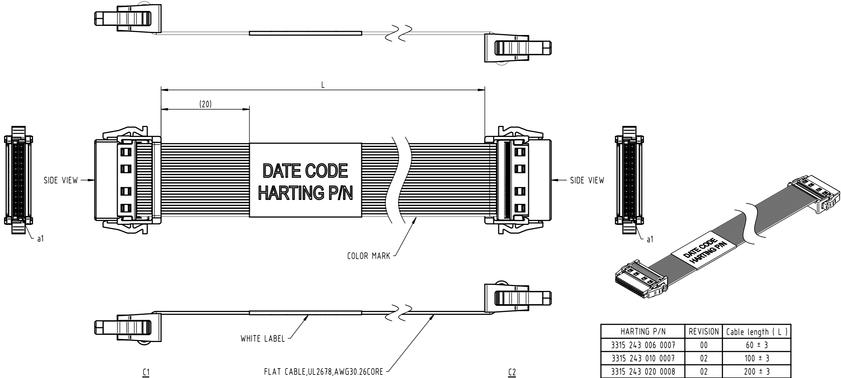
C1 HAR-FLEX 26 POLE FEMALE CONNECTOR WITH STRAIN RELIEF
