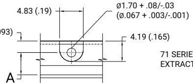
MOUNTING HOLE DETAIL NOT TO SCALE
