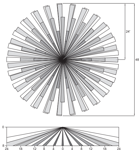
Sensor Lens Coverage and Detection Patterns When Mounted at 8ft with Low Mount Lenses
