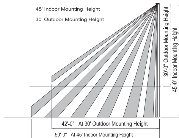
Sensor Lens Coverage and Detection Patterns When Mounted at 30ft and 45ft with Standard Lenses
