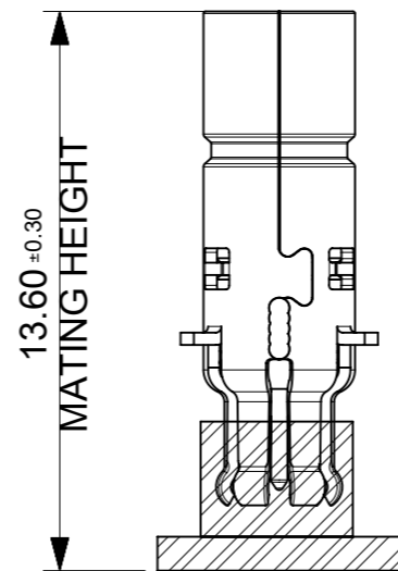
PCB WITH JACK(2087941005)
