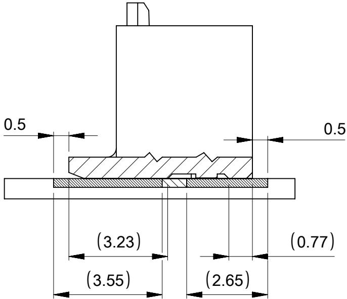
SECTION Z-Z
