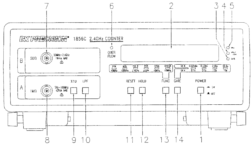
Figure 1. Front Panel
