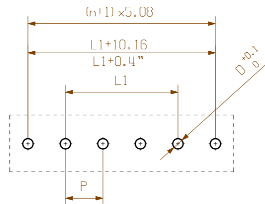
HOLE PATTERN
