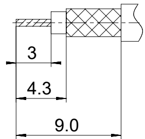
Cable trimming dimensions
