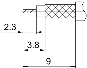
Cable trimming dimensions
