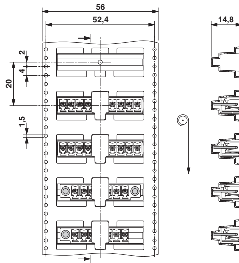
Dimensioned drawing
