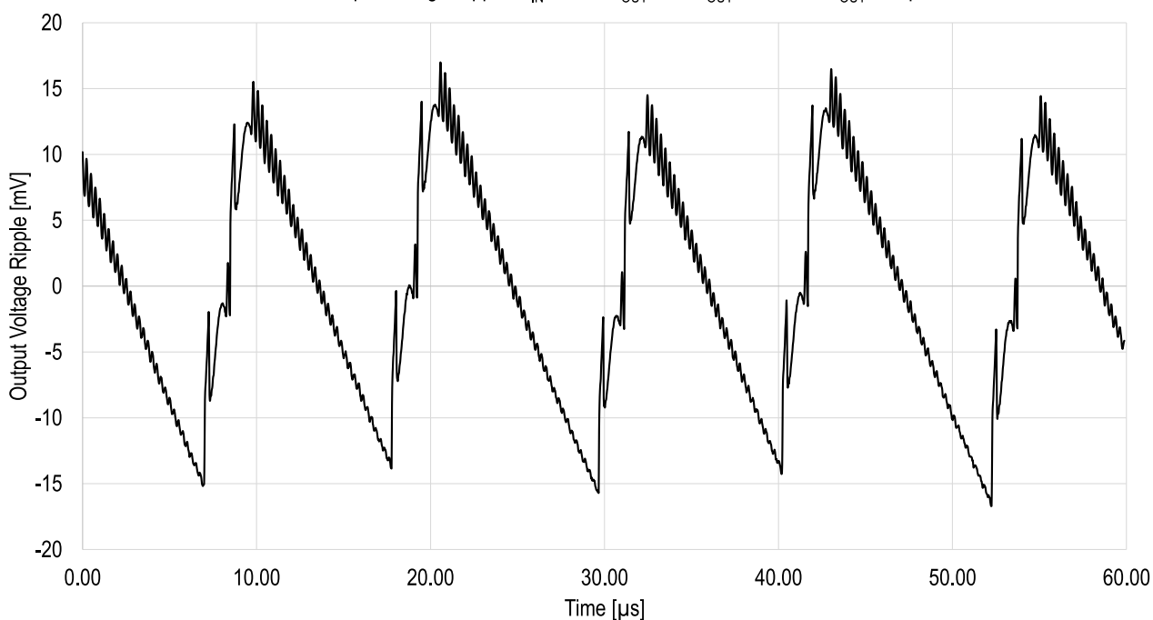
171013801 Output Voltage Ripple, V_{IN} = 24V , V_{OUT} = 12V , I_{OUT} = 100mA , C_{OUT} = 22\mu F
