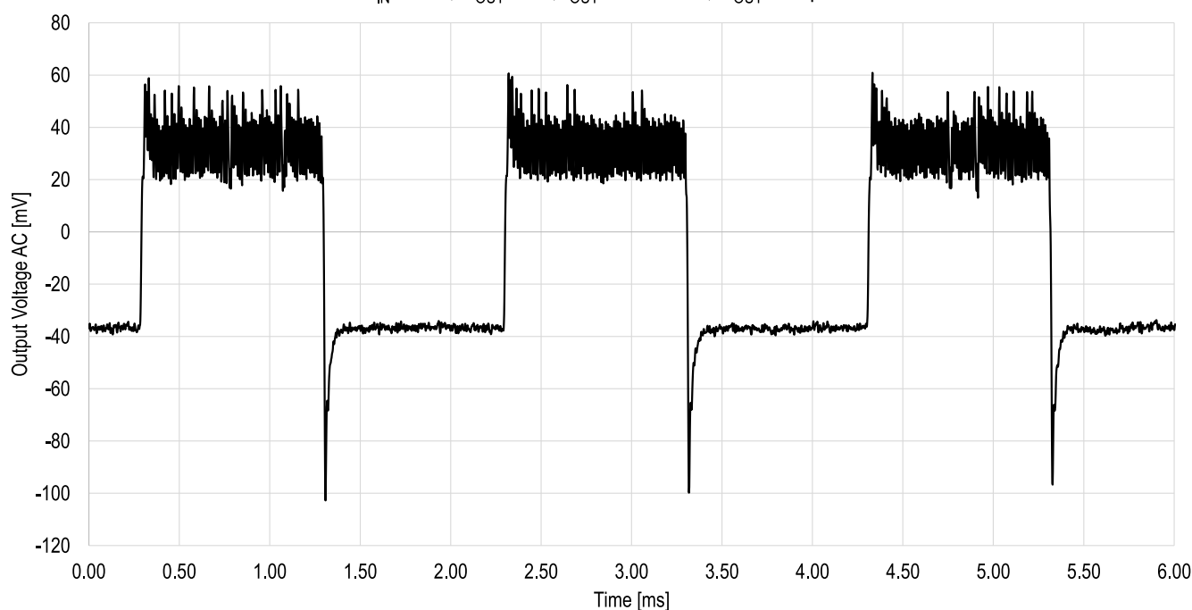
171013801 Output Voltage Load Transient Response
